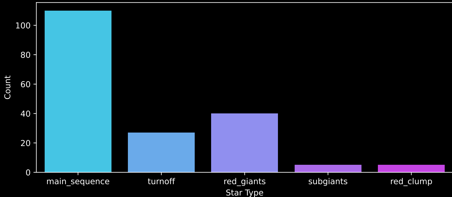
APOGEE DR17 Field: [110+61_MGA] Count plot of Star Type
