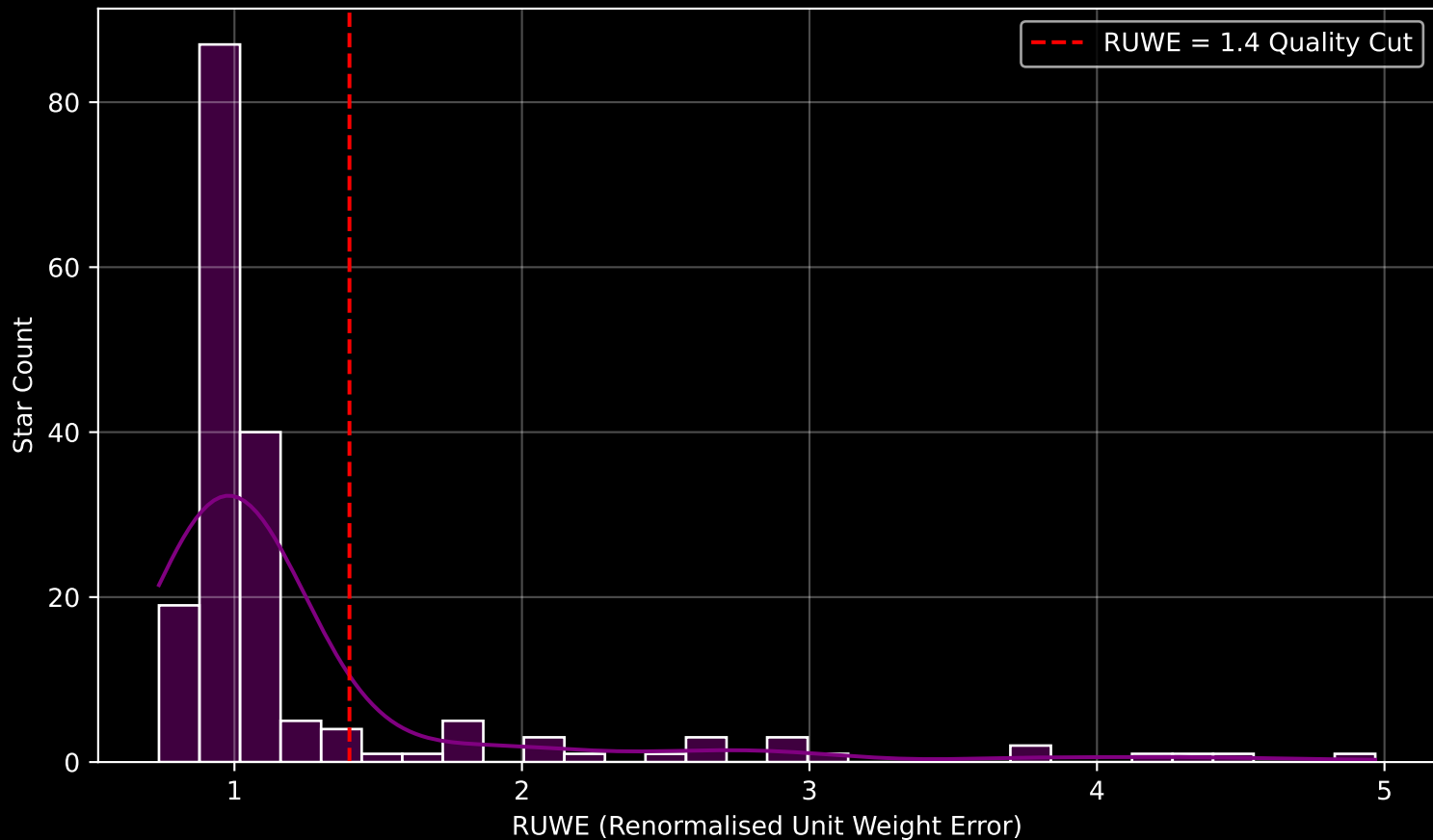
GAPOGEE DR17 Field [110+61_MGA] RUWE Distribution (n= 180)
