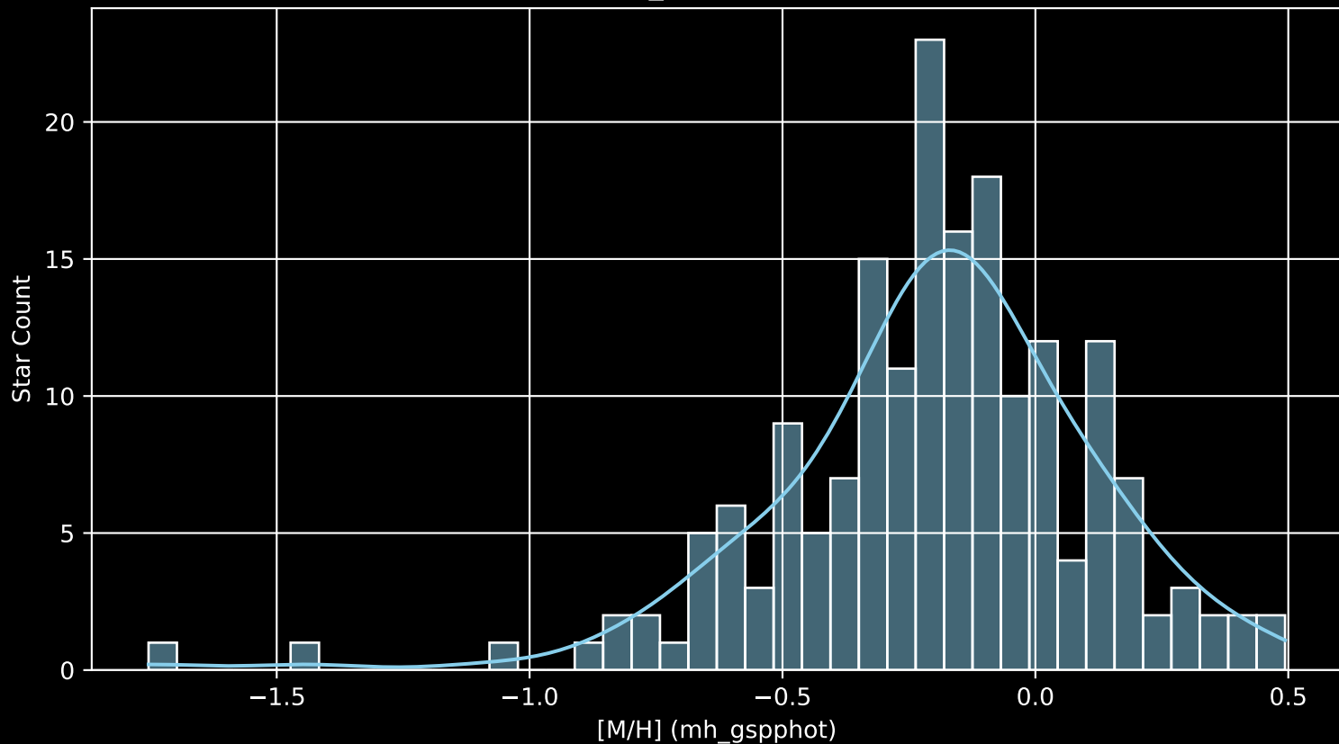
APOGEE DR17 Field: [110+61_MGA [M/H] (mh_gspphot) (n= 183)
