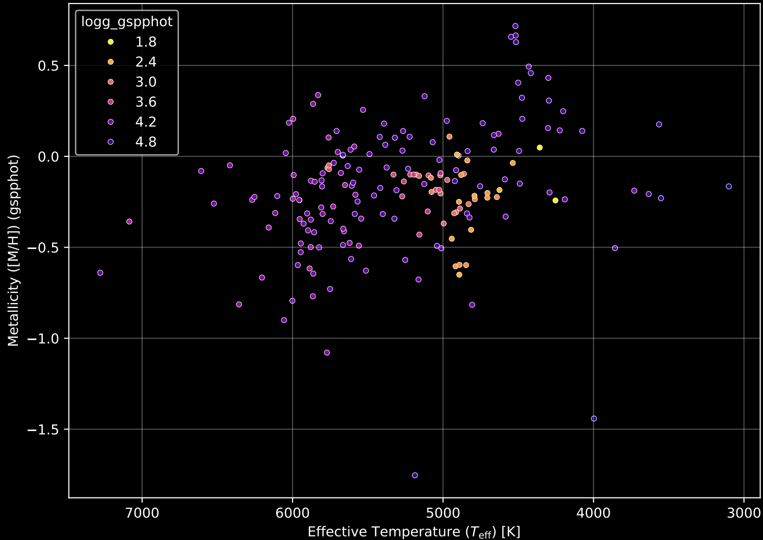
APOGEE DR17 Field: [110+61_MGA] Stellar Population Parameters (n= 187)
