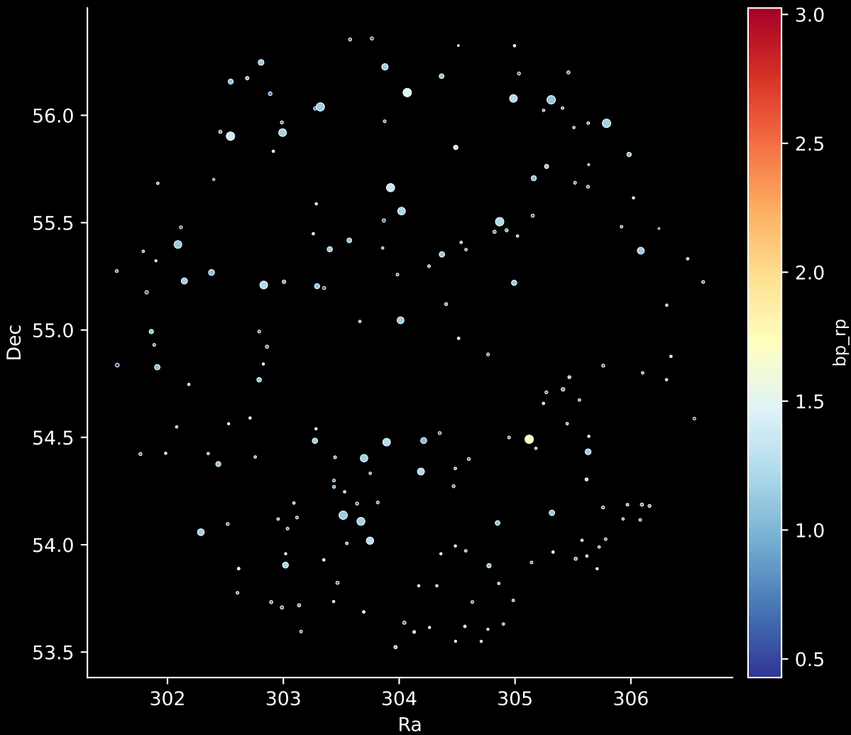
APOGEE DR17 Field: [110+61_MGA] Stars: 187
