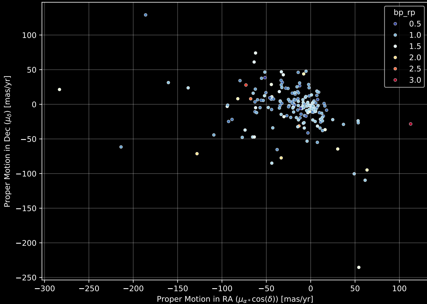
APOGEE DR17 Field: [110+61_MGA] Proper Motion Diagram (n= 187)
