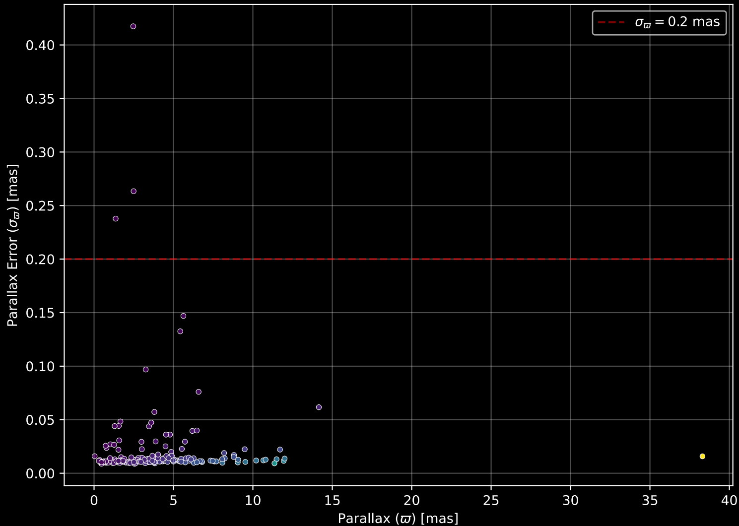
APOGEE DR17 Field: [110+61_MGA] Parallax Quality (n= 187)
